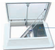
Grid with ladder brace Comfort safety roof exit with grid and ladder brace according BG rules
